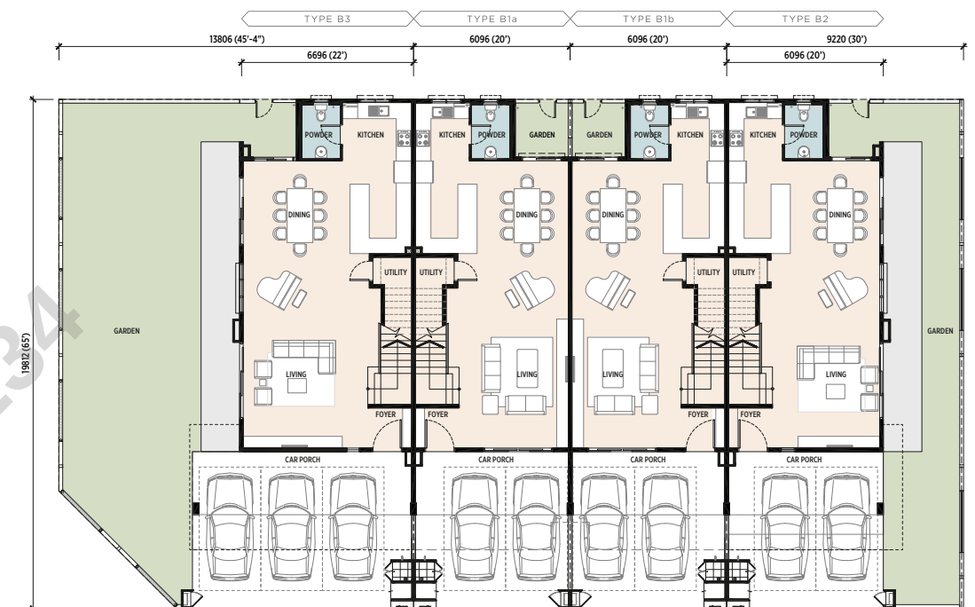
GROUND FLOOR
