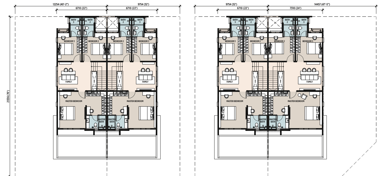
FIRST FLOOR
