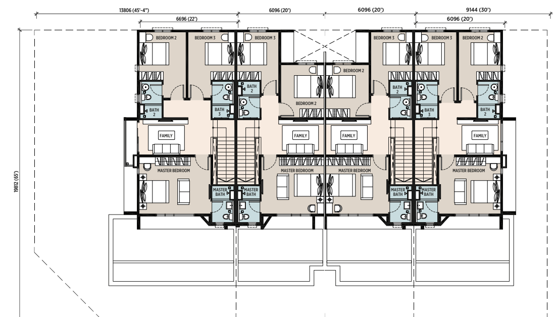
FIRST FLOOR
