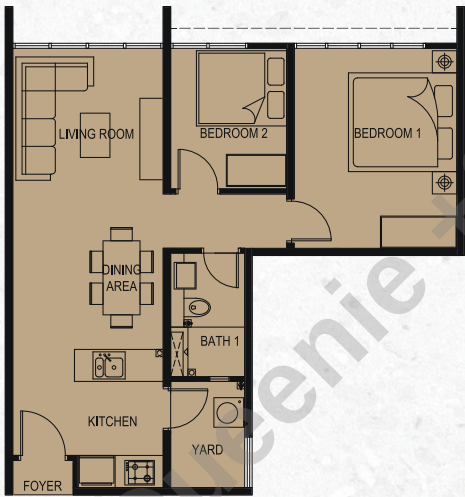
TYPE B1 660 SQ.Ft. 2 Bedrooms 1 Bathroom
